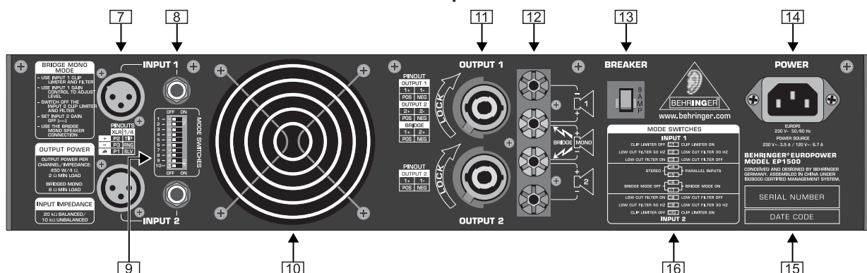
Fig. 2.2: Rear panel control elements
